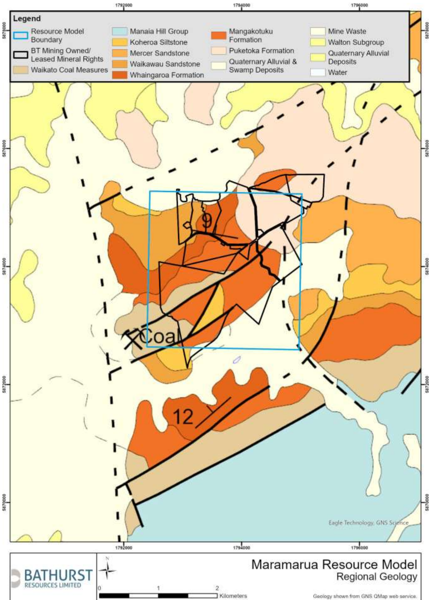
Figure 2: Regional Geology
