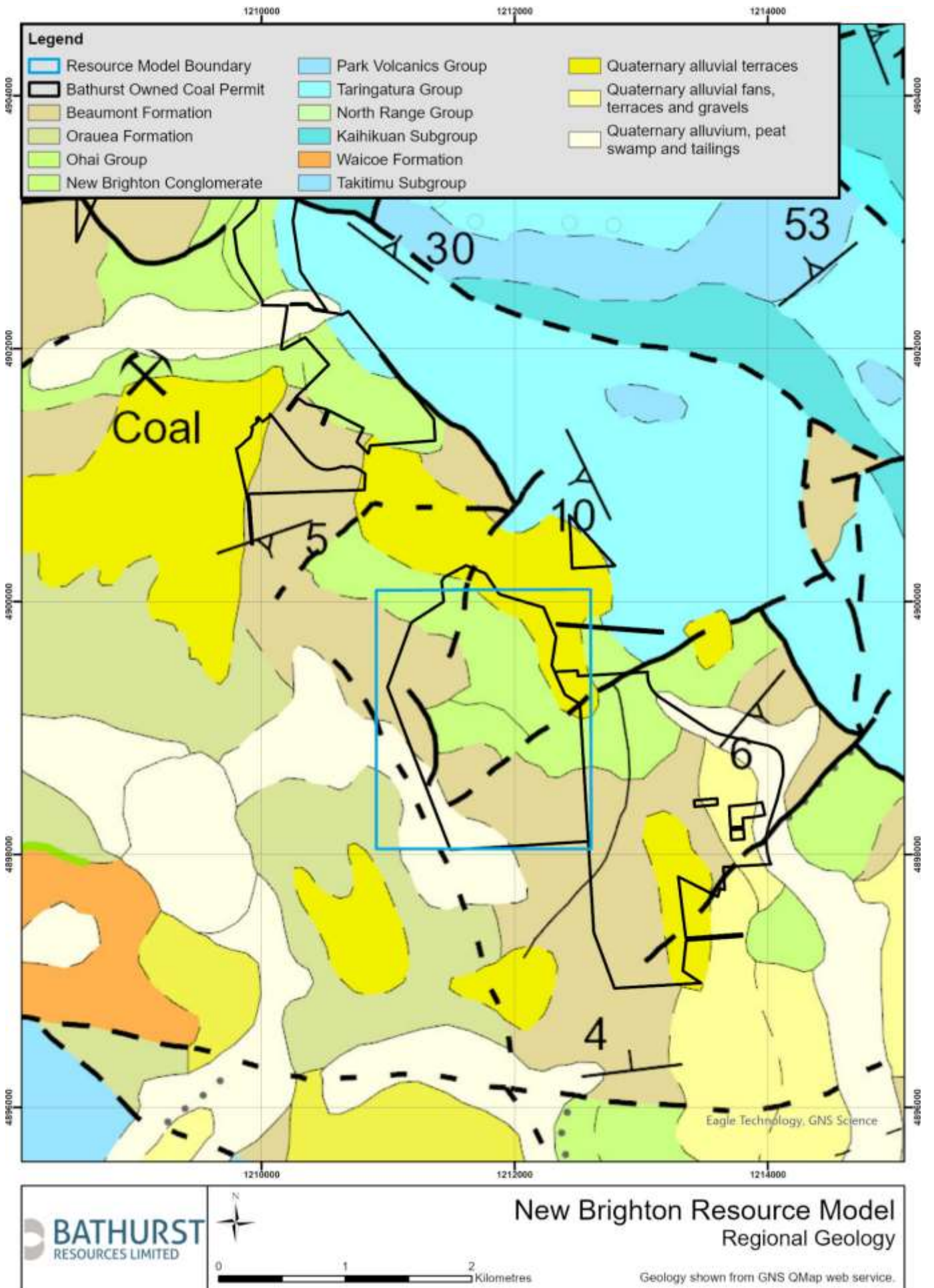
Figure 2: Regional Geology
