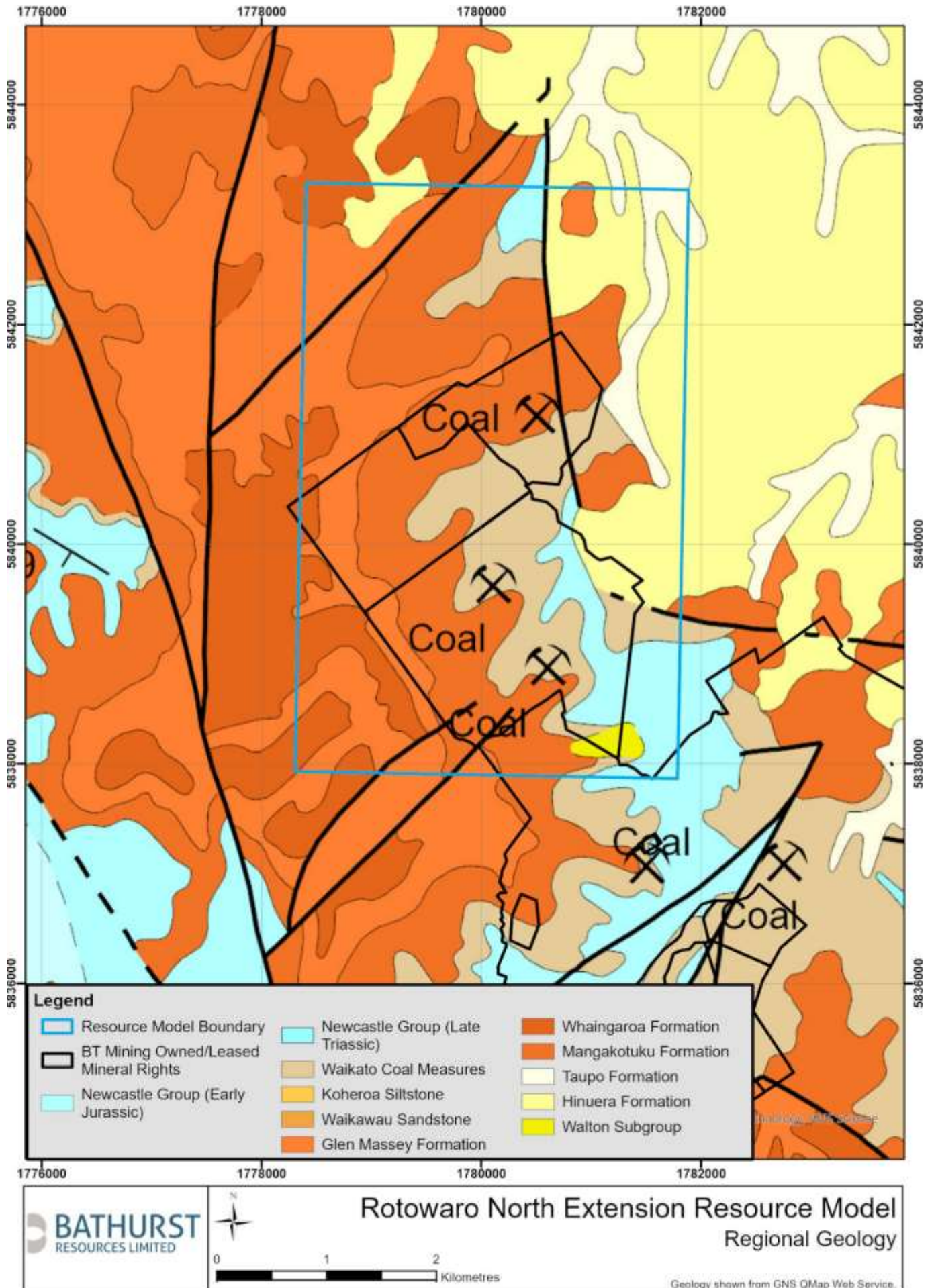
Figure 2: Regional Geology
