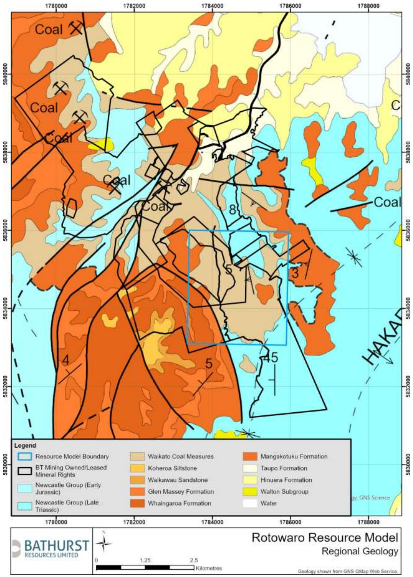
Figure 2: Regional Geology
