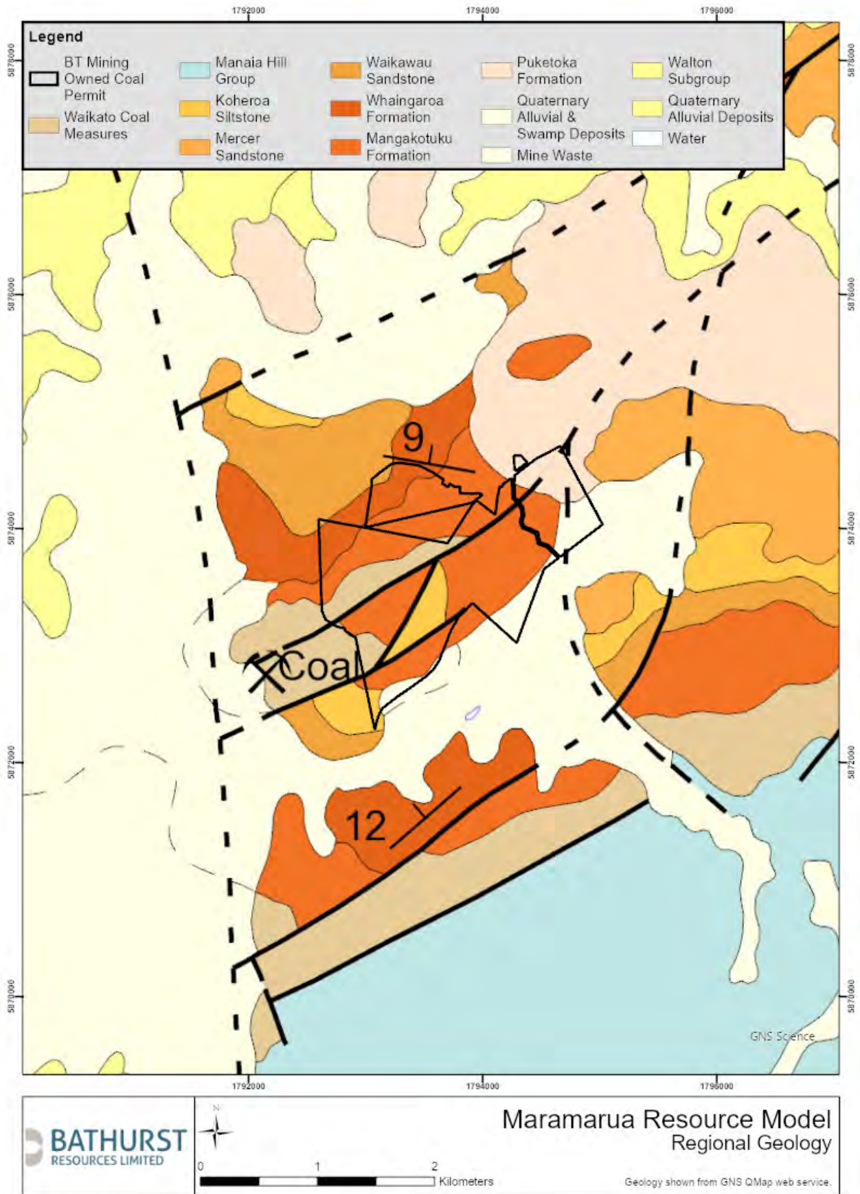
Figure 2: Regional Geology
