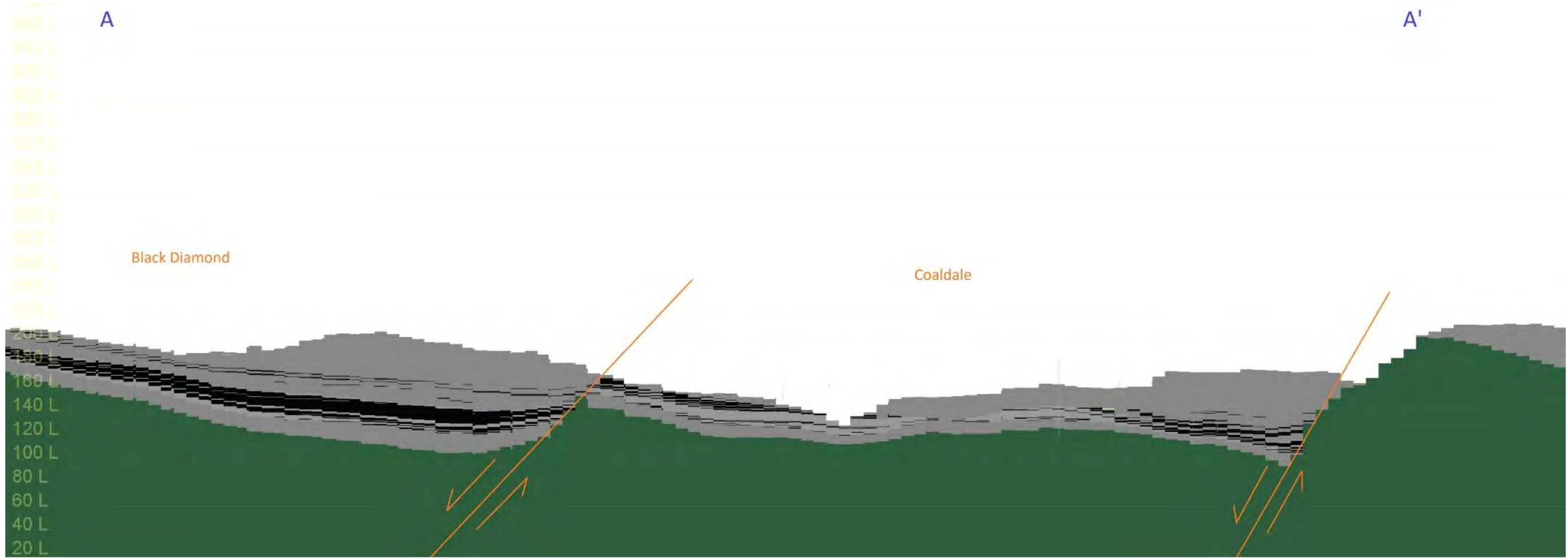
Figure 22: Section view through the deposit. The Black Diamond south fault and Trig E faults are shown
