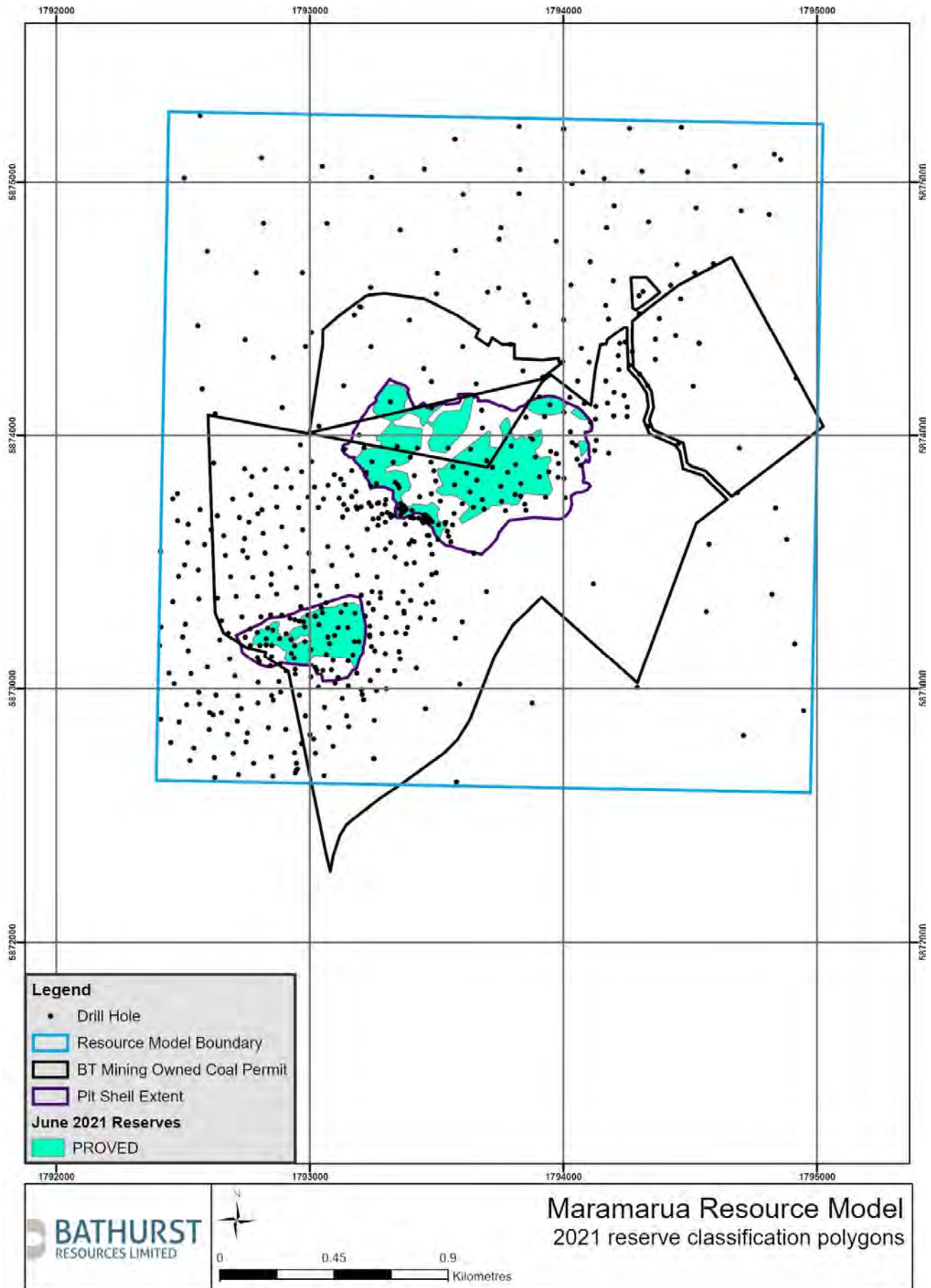
Figure 11: Mamarua reserve classification polygons with pit shell extents
