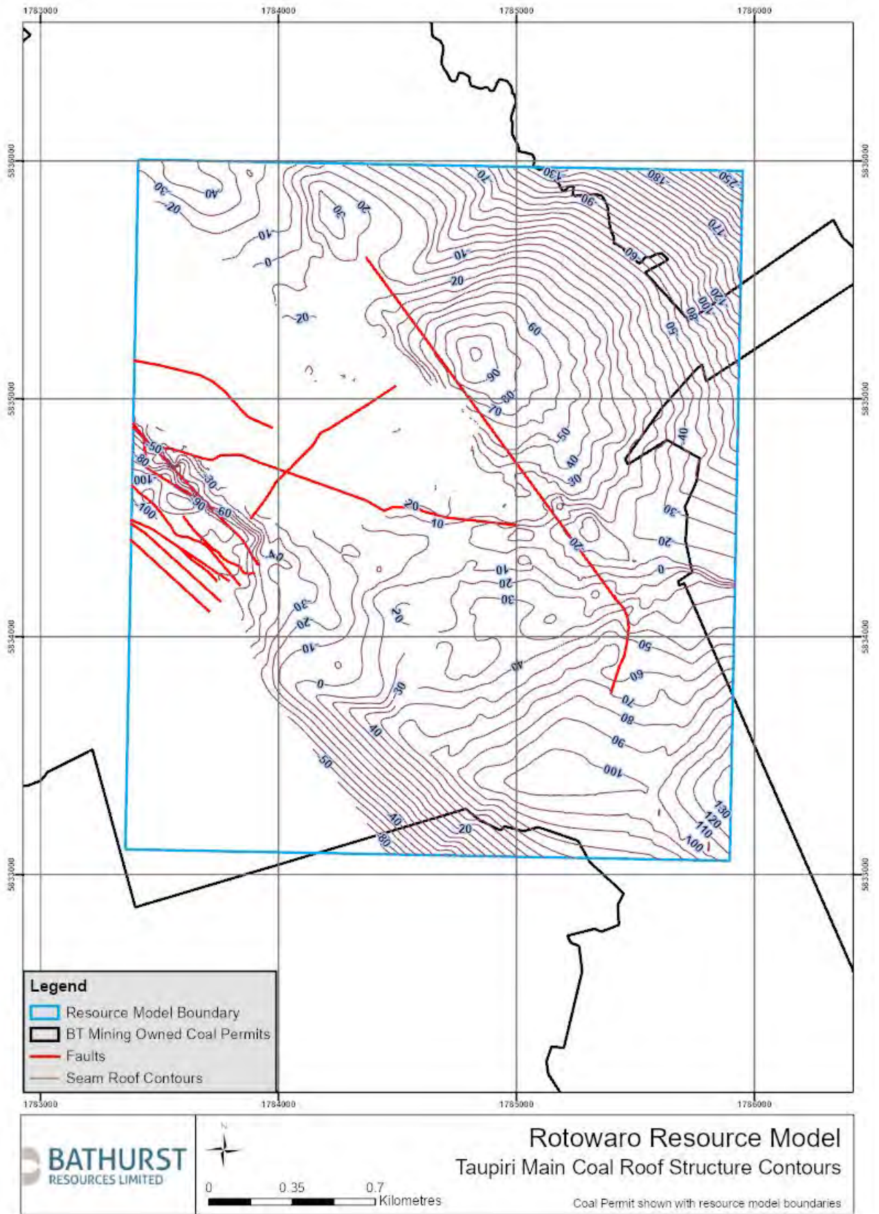
Figure 7: Plan showing the structure contours of coal seam roof
