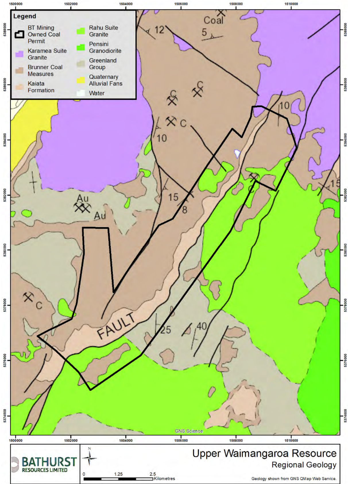
Figure 3: Regional Geology
