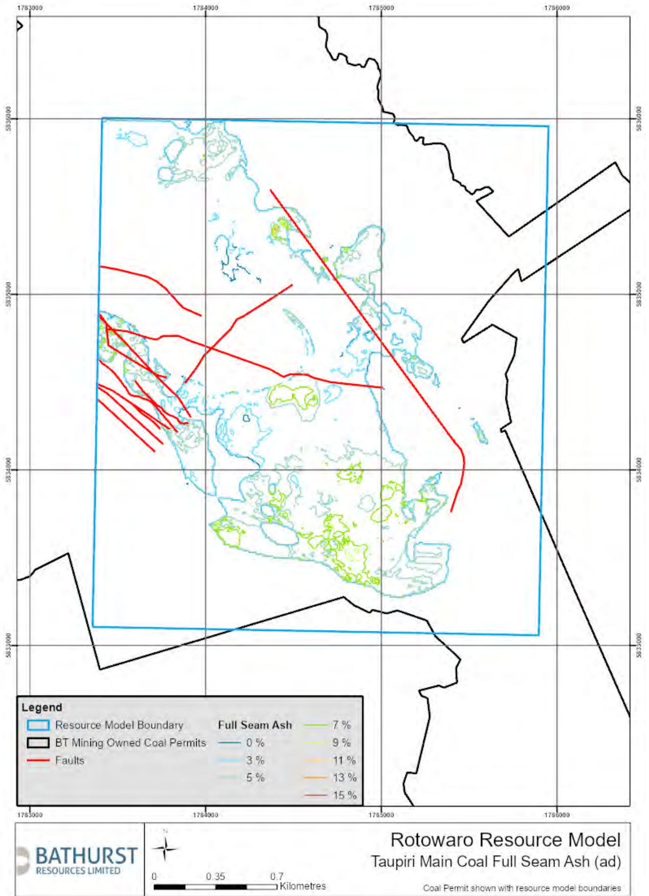
Figure 9: Plan showing in situ full seam ash on an air-dried basis as modelled over the deposit area
