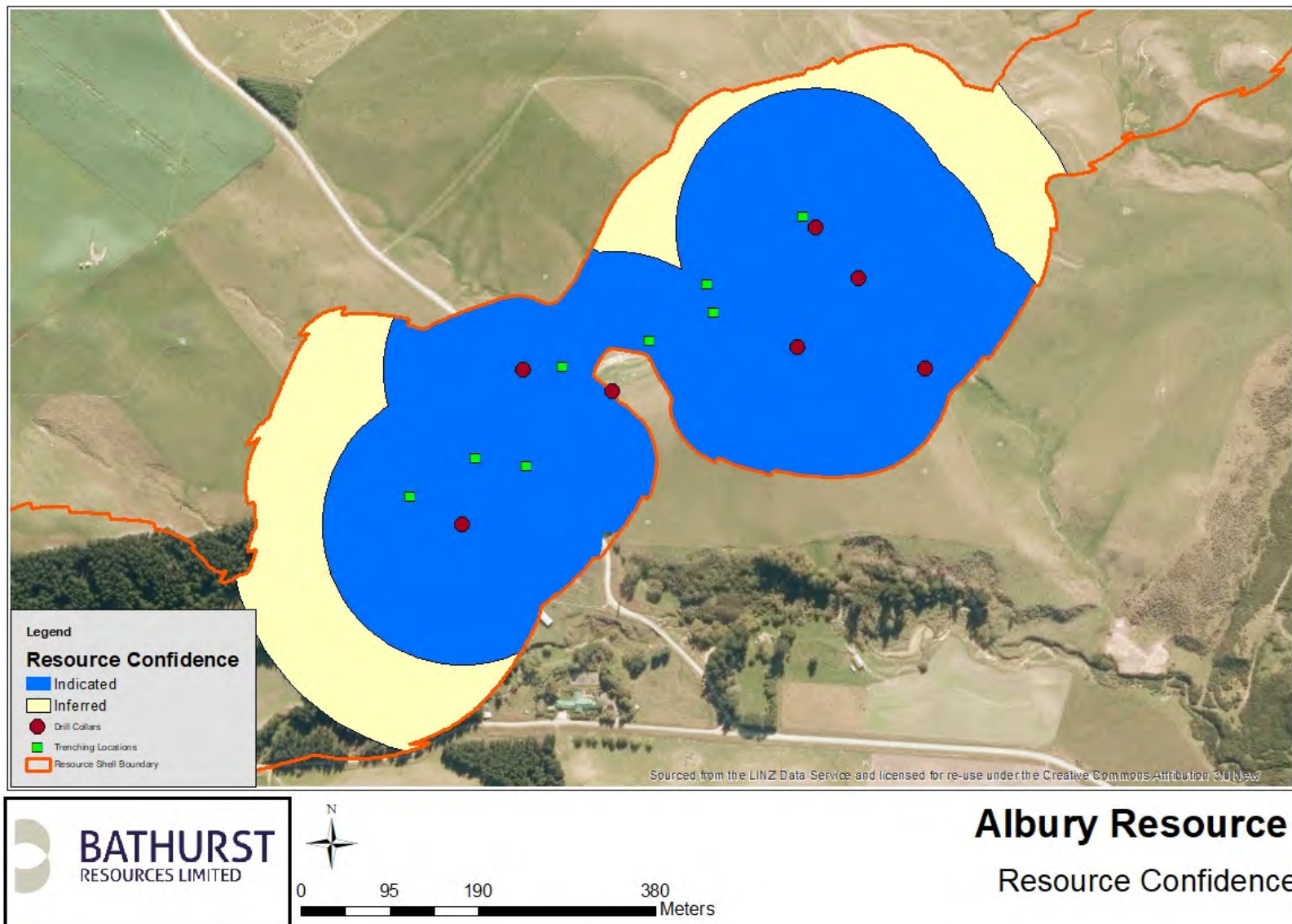
Figure 6: Resource Confidence
