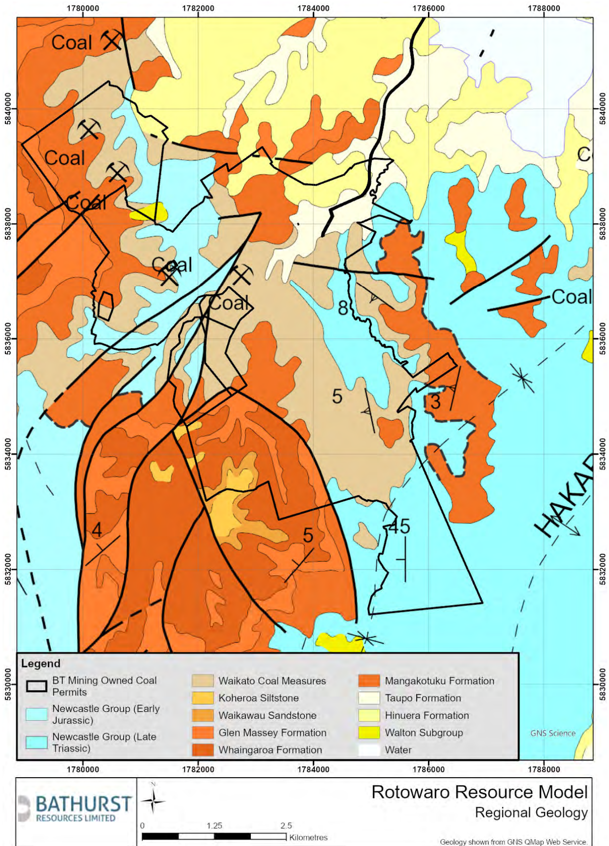
Figure 2: Regional Geology
