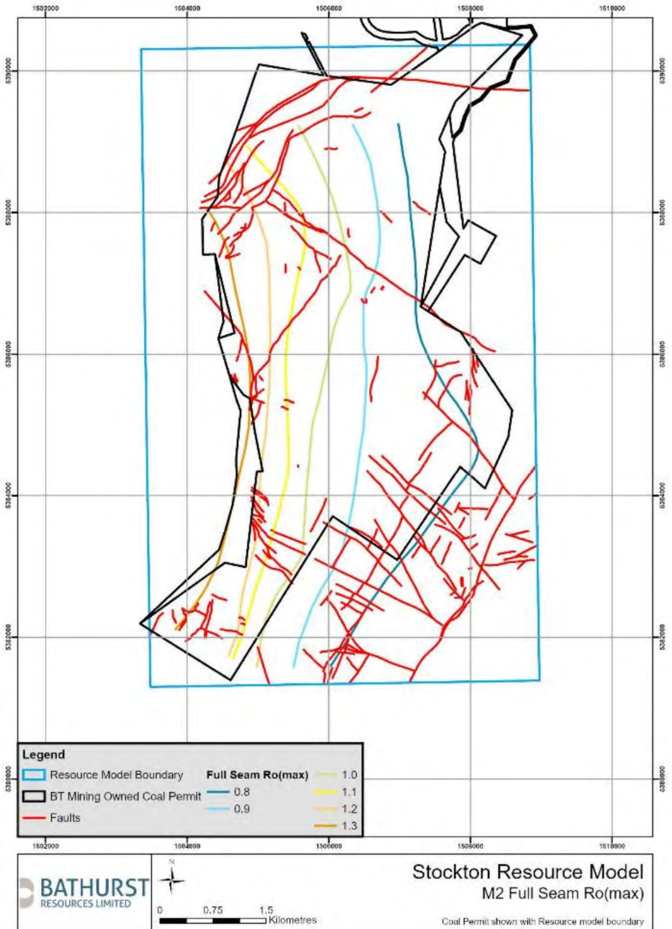
Figure 11: Map showing M2 RO(MAX) distribution
